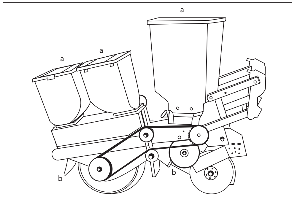
Figure 7: Granule applicator
