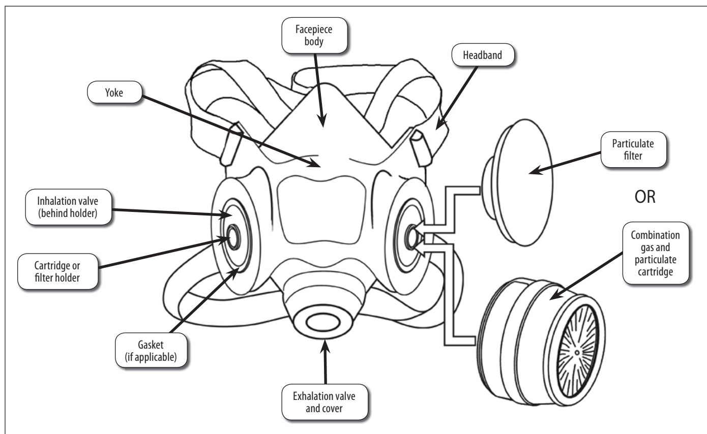
Figure 11: Diagram of a cartridge respirator
