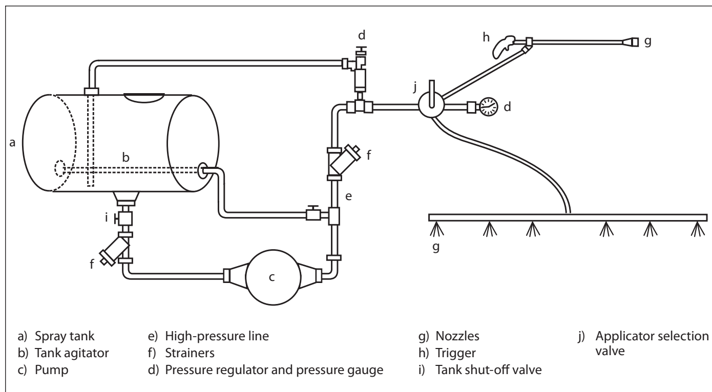
Figure 10: Hydraulic sprayer
