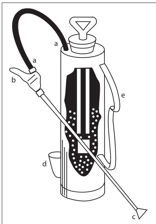
Figure 8: Hand sprayer
